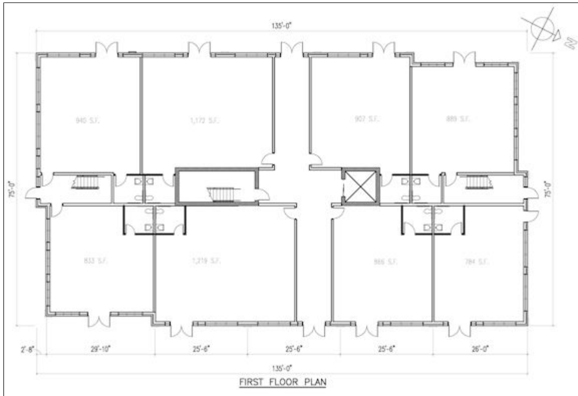
Plan 1: First Floor Plan
